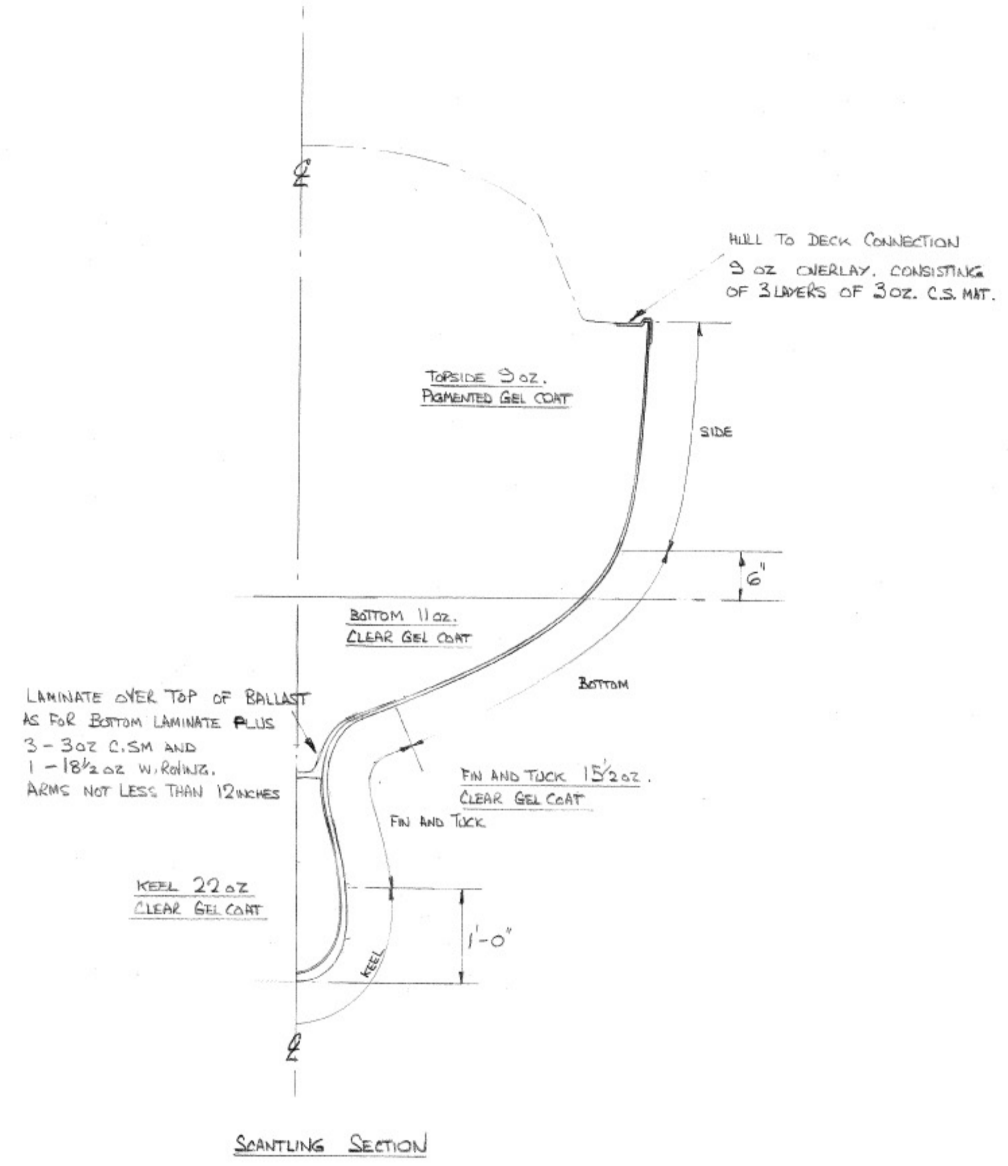
SCANTLING SECTION
